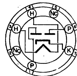
BOTTOM VIEW MINIATURE BUTTON 7 PIN BASE 5BS
